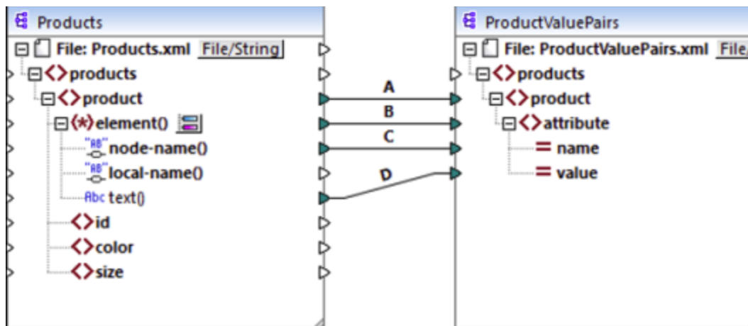
ConvertProducts.mfd
