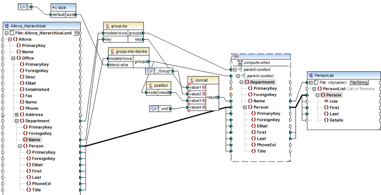
DividePersonsByDepartmentIntoGroups.mfd
