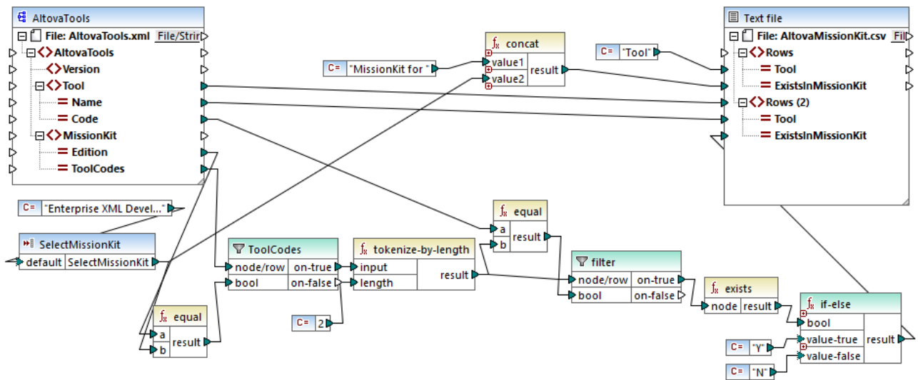
tokenizeString2.mfd
