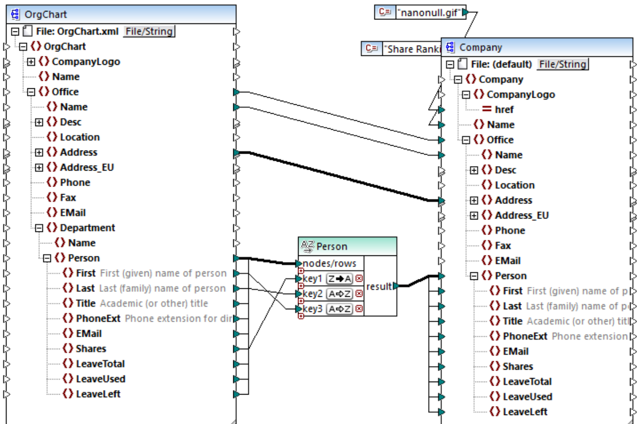
SortByMultipleKeys.mfd
