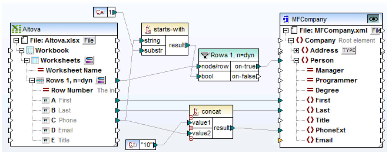
Excel-mapping.mfd (sample 1)
