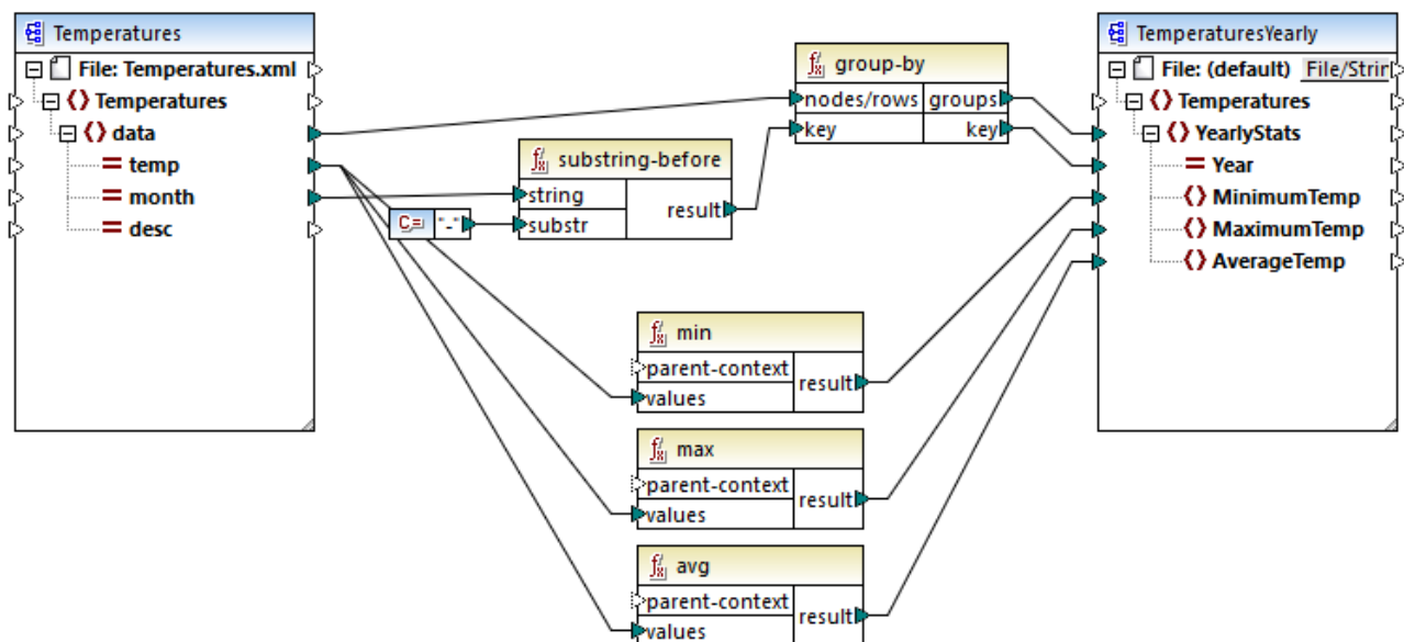
GroupTemperaturesByYear.mfd
