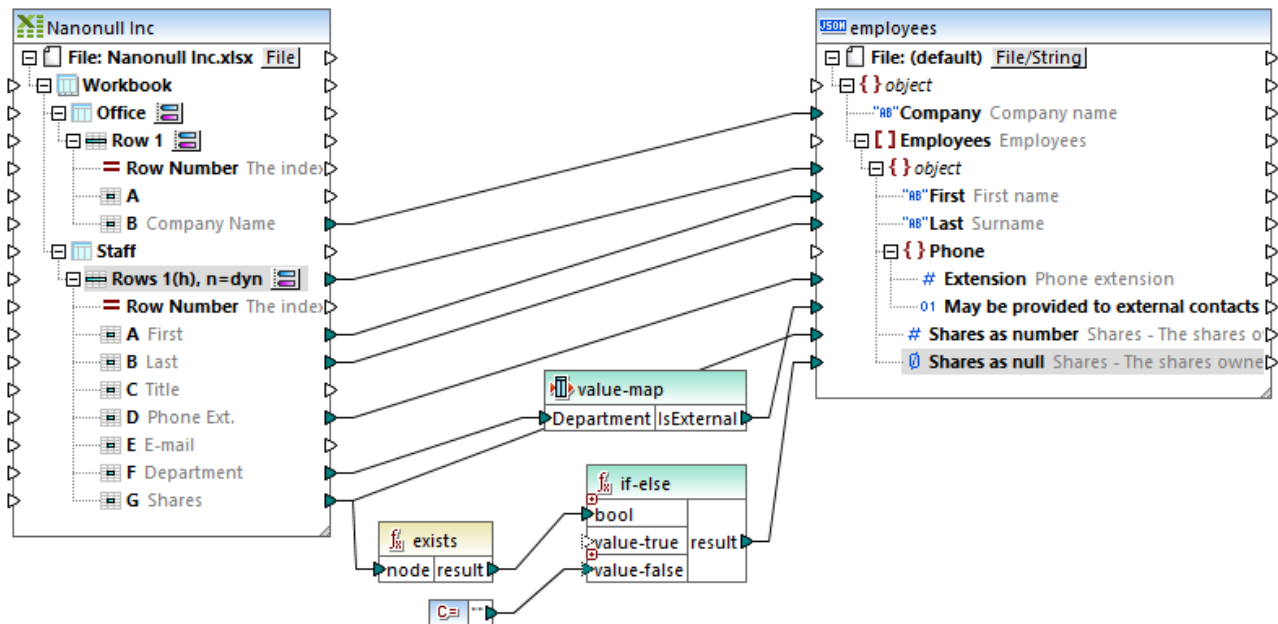
Excel_Company_To_JSON.mfd
